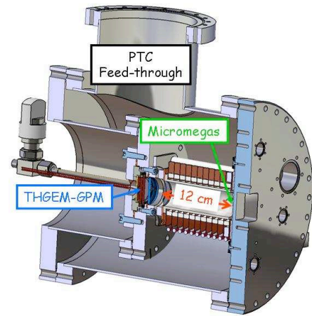
FIG. 83 Schematic of the Nantes LXe Compton PET prototype (Grignon, 2007).
