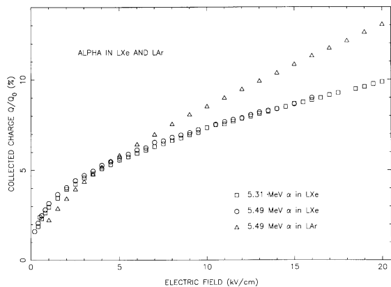
FIG. 3 Collected charge ( Q/Q_0 %) as a function of electric field for ^{210}\text{Po} in liquid xenon (squares) and ^{241}\text{Am} in liquid xenon (circles) and liquid argon (triangles)(Aprile, 1991b).
