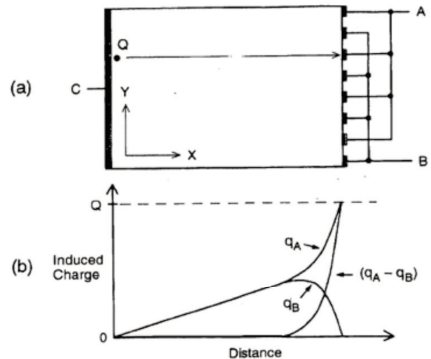
FIG. 32 (a) Schematic of an ionization chamber with a coplanar anode made of parallel strips (Luke, 1995). (b) Time variation of the induced charge signals and the resulting signal in case the charge Q is collected onto the group of strips marked as A.
