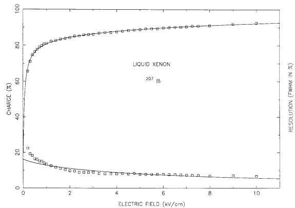
FIG. 4 Collected charge and energy resolution of 570 keV gamma-rays in LXe as a function of electric field (Aprile, 1991a).
