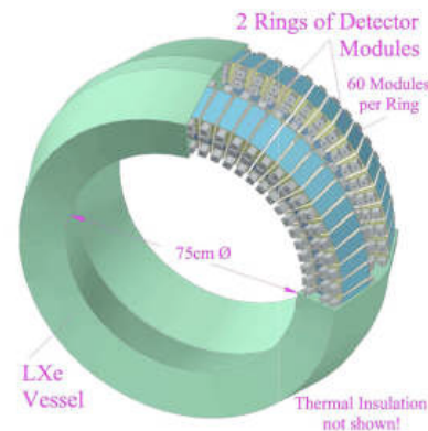
FIG. 82 Schematic of the Columbia full scale LXe Compton PET (Giboni, 2007).
