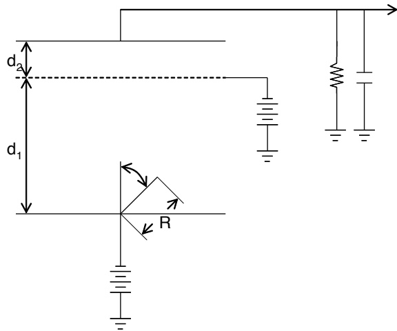
FIG. 30 Schematic drawing of a gridded ionization chamber.
