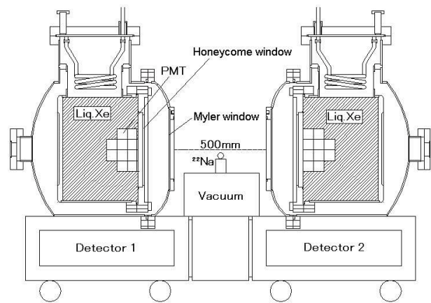
FIG. 85 Schematic of the Waseda TOF PET prototype (Nishikido, 2004).
