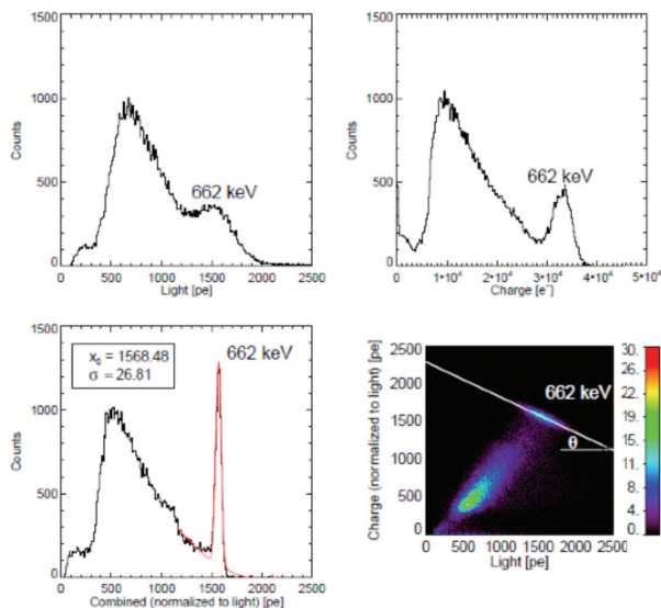
FIG. 42 Energy spectra of \text{Cs}^{137} 662 keV \gamma -rays measured with 1 kV/cm field in LXe, separately from charge and light (top panels) and from combined charge and light (lower panel, left); charge-light anti-correlation and its angle (lower panel, right) (Aprile, 2007b).
