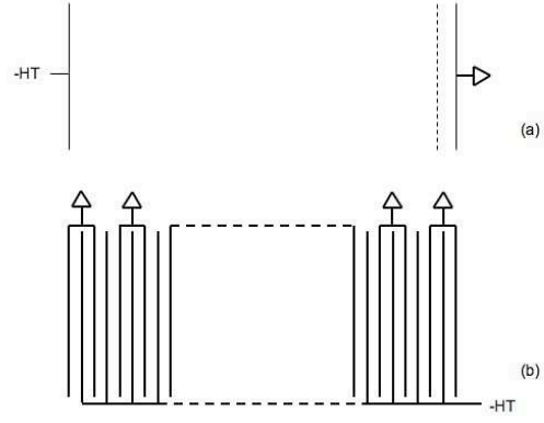
FIG. 36 (a) Gridded ionization chamber with a long sensitive region. (b) Multi-parallel plate electrode system for an ionization calorimeter (Doke, 1993).
