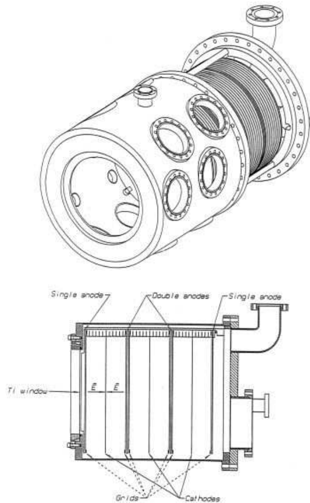
FIG. 73 (top) Schematic of the RAPID LXeTPC vessel with Ti window for incident \gamma -rays and quartz windows for PMTs. (bottom) Cross section of the electrodes for charge read out (Bressi, 1998).
