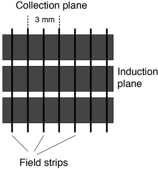
FIG. 33 An example of two-dimensional position-sensitive electrode, with orthogonal strips for collection and induction signals (Cennini, 1994).
