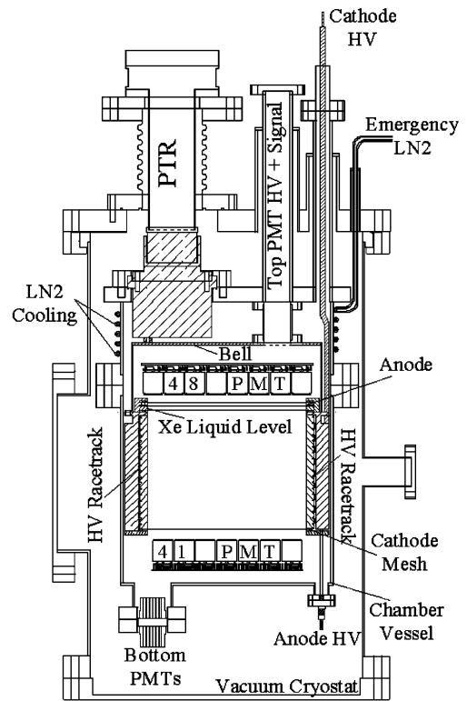
FIG. 54 Schematic of the XENON10 detector (Aprile, 2009).
