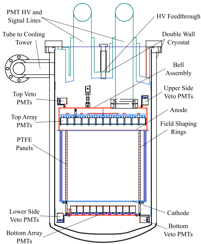
FIG. 56 Schematic of the XENON100 detector (Aprile, IDM08 Proceedings).
