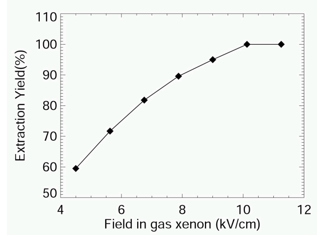
FIG. 46 Electron-extraction yield in LXe as a function of the electric field in the gas phase (Aprile, 2004).
