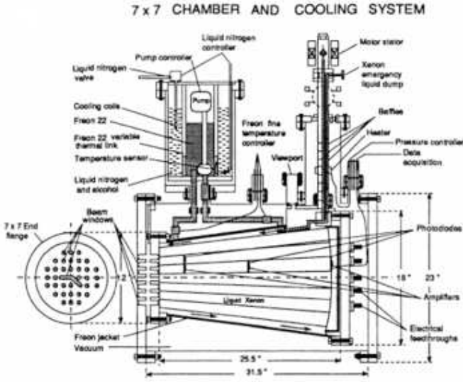
FIG. 70 Schematic of the MIT-ITEP-Dubna LXe scintillation calorimeter prototype (Akimov, 1996).
