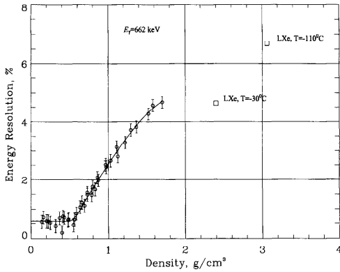
FIG. 8 Density dependence of the energy resolution (%FWHM) measured for 662 keV \gamma -rays (Bolotnikov, 1997).
