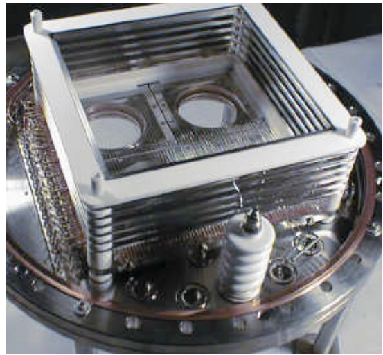
FIG. 49 The LXeGRIT TPC structure (cathode removed) (Aprile, 2003b).
