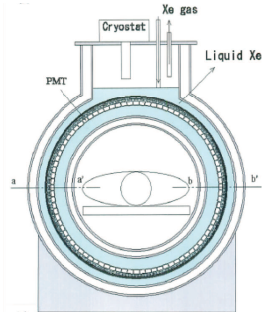
FIG. 87 Schematic of the Waseda full scale LXe TOF-PET (Doke, 2006).
