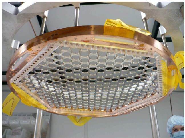
FIG. 78 Image of one EXO-200 anode plane. Induction and charge collection grids cross at 120^\circ . The LAAPD support platter is visible behind the grids. (Gratta, 2009).
