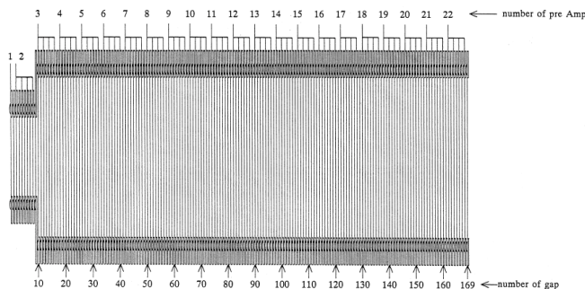
FIG. 67 Schematic of the Waseda multi-plate LXe ionization calorimeter (Okada, 2000).
