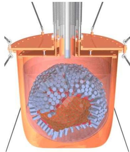
FIG. 63 Schematic of the XMASS detector (Suzuki, IDM08 Proceedings).
