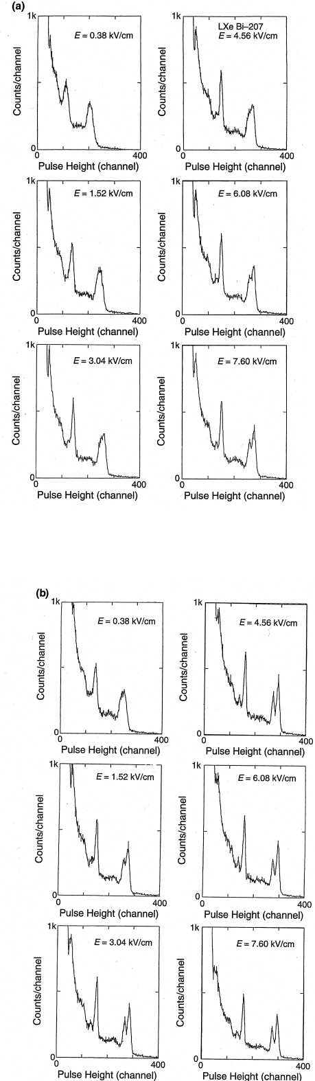
FIG. 17 Comparison between the energy spectra of ^{207}\text{Bi} internal conversion electrons and gamma-rays measured from ionization (a) in pure liquid xenon and (b) in TEA-doped liquid xenon.
