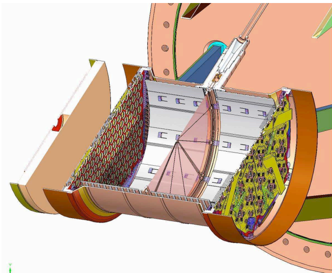
FIG. 77 Schematic of the EXO-200 TPC (Gratta, 2009).
