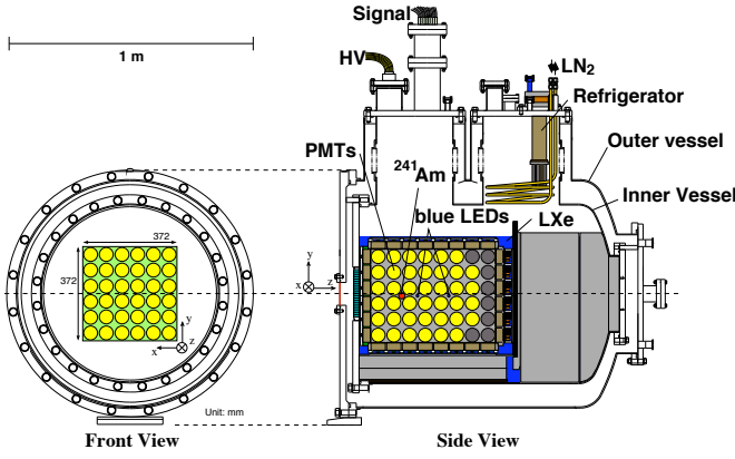
FIG. 74 Schematic of the large MEG prototype (Mihara, 2004a).
