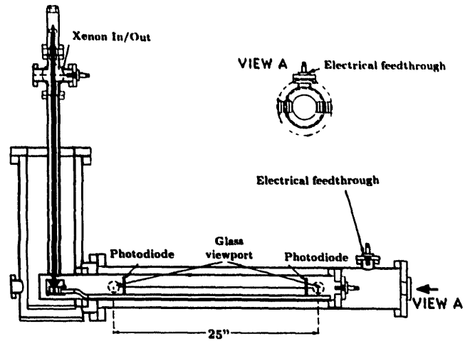
FIG. 68 Schematic of a full length liquid xenon/krypton cell for uniformity tests with mirrors and diodes (Chen, 1993).
