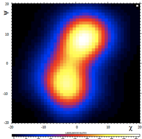
FIG. 50 LXeGRIT image of two calibration sources, ^{60}\text{Co} and ^{22}\text{Na} , using a maximum likelihood imaging technique. Reprinted with permission from (Aprile, 2008a).
