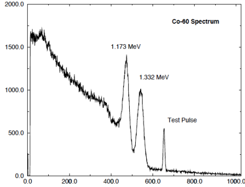
FIG. 35 The energy spectrum of Co 60 gamma-rays measured with a gridded ionization chamber (Aprile, 2001).
