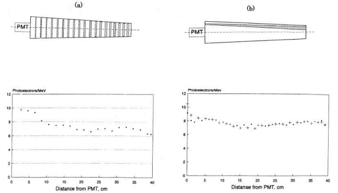
FIG. 72 Efficiency of light collection measured with the movable alpha-source. Crosses (curves) are measured (Monte Carlo simulated) for the cell illustrated in Figure 71 (Akimov, 1996)
