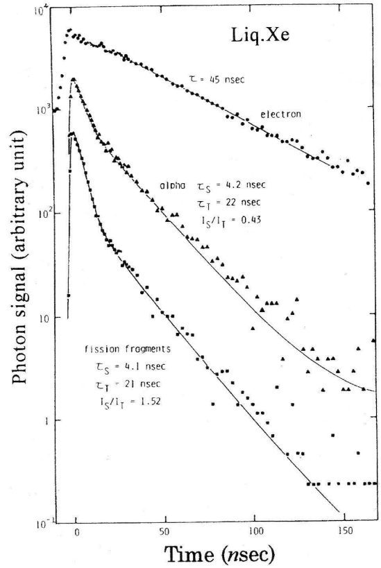
FIG. 19 Decay curves of scintillation from liquid xenon excited by electrons, \alpha -particles and fission fragments, without an applied electric field (Hitachi, 1983; Kubota, 1978a).
