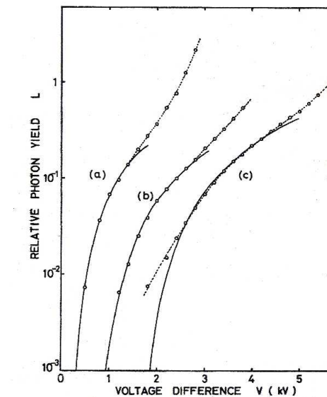
FIG. 14 Relative photon yield of proportional scintillation and charge gain as a function of applied voltage to anode wires of different diameter. Solid lines are results of the fit in (Derenzo, 1974) to the data points in the region of the ionization chamber mode: (a) for 4 \mu\text{m} diameter wire, (b) for 10 \mu\text{m} , (c) for 20 \mu\text{m} (Masuda, 1979).
