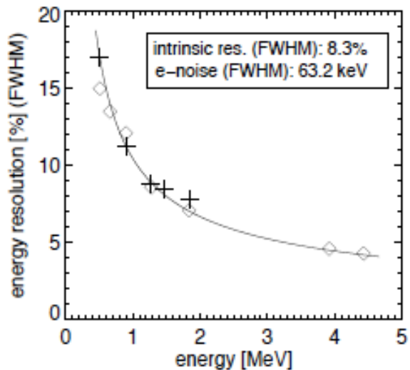
FIG. 51 The energy resolution of LXeGRIT as a function of energy.
