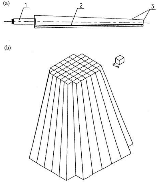
FIG. 71 (a) Unit cell of the LXe scintillation calorimeter:(1) PMT, (2) fragment of p-terphenyle strip, (3) Mylar reflector. (b) Assembly of the full calorimeter reflector structure (Akimov, 1995).
