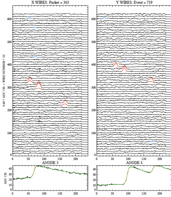
FIG. 43 Display of a 1.8 MeV \gamma -ray event with multiple Compton interactions, recorded with the LXeTPC (Aprile, 1998).
