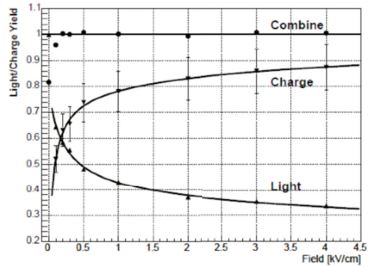
FIG. 41 Light and charge as a function of drift field for ^{137}\text{Cs} 662 keV \gamma -rays (Aprile, 2007b).
