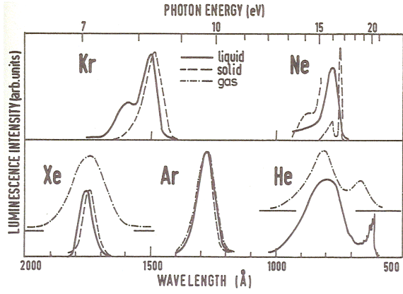
FIG. 18 Emission bands in liquid rare gases, together with solid- and gas-phase spectra (Jortner, 1965; Schwenter, 1985).
