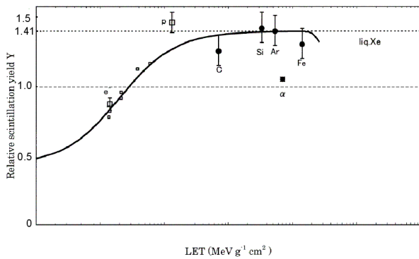
FIG. 23 LET dependence of the scintillation yield in liquid xenon for various ionizing particles (Doke, 2002; Tanaka, 2001).
