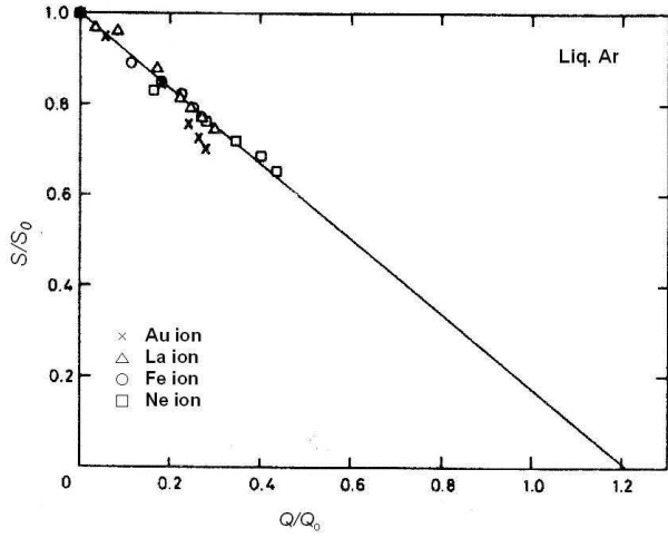
FIG. 26 Anti-correlation between scintillation intensity and collected charge in liquid argon for relativistic Ne ions(□), Fe ions (o), La ions (Δ ), and Au ions (x). The solid line is the theoretically estimated relation (Masuda, 1989).
