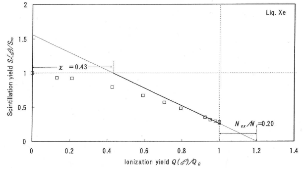
FIG. 29 Relation between S_r/S_{r0} and Q/Q_0 in liquid xenon (Doke, 2002).
