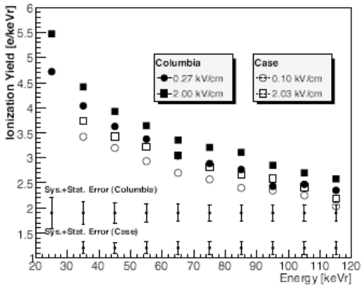
FIG. 5 Ionization yield from nuclear recoils measured with small scale two-phase xenon detectors (Aprile, 2006).
