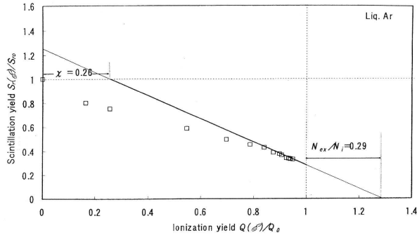
FIG. 28 Relation between S_r/S_{r0} and Q/Q_0 in liquid argon (Doke, 2002).
