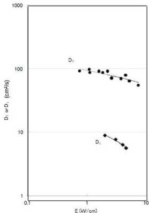
FIG. 12 Transverse and longitudinal diffusion coefficients for electrons in LXe as a function of electric field (Doke, 1981; Shibamura, 2009).
