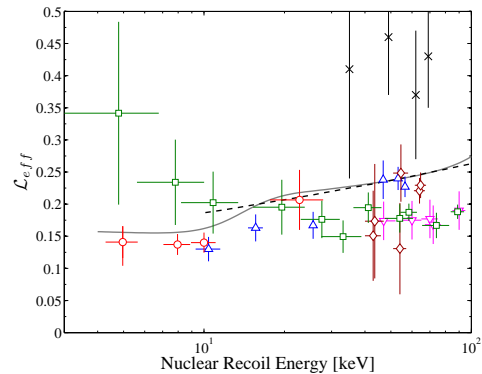
FIG. 24 Relative scintillation efficiency of nuclear recoils in LXe (Aprile, 2008c) and references therein.
