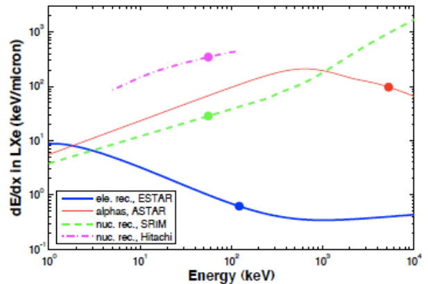
FIG. 7 Predicted electronic stopping power, dE/dx , for different particles in LXe. The circles refer to the particle energies discussed in (Aprile, 2006).
