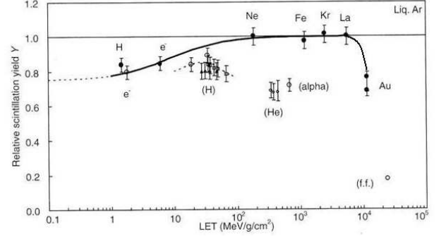
FIG. 21 LET dependence of the scintillation yield in liquid argon for various ionizing particles (Doke, 1988, 2002).
