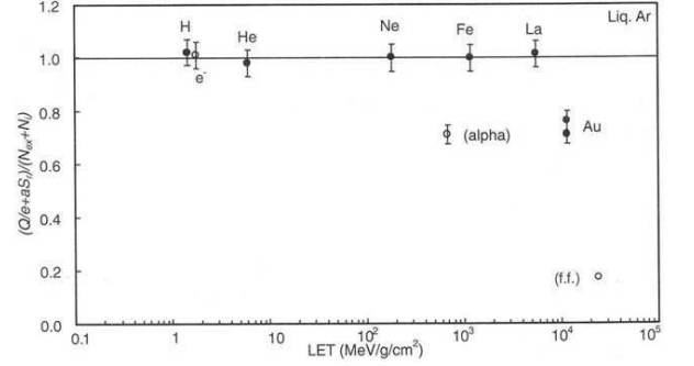
FIG. 22 LET dependence of the ratio (Q/e + aS_n)/(N_{ex} + N_i) in liquid argon. The label (f.f.) stands for fission fragments or non-relativistic particles (Doke, 1988, 2002).
