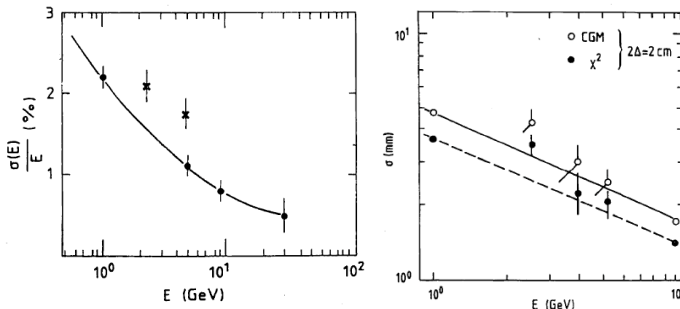
FIG. 66 Energy (left) and position (right) resolution dependence on electron energy ( \times are the experimental points and \circ are points from Monte Carlo simulations (Baranov, 1990).
