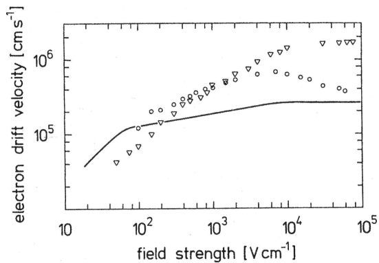
FIG. 10 Influence of butane on the electron drift velocity in liquid xenon. Butane ( \circ : 0.09%), ( \Delta : 1.4%), and solid line: pure xenon (Yoshino, 1976).
