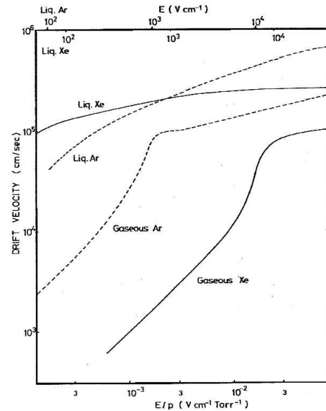
FIG. 9 Electron drift velocity in gaseous and liquid xenon and argon, as a function of reduced electric field (Miller, 1968; Pack, 1962; Yoshino, 1976).
