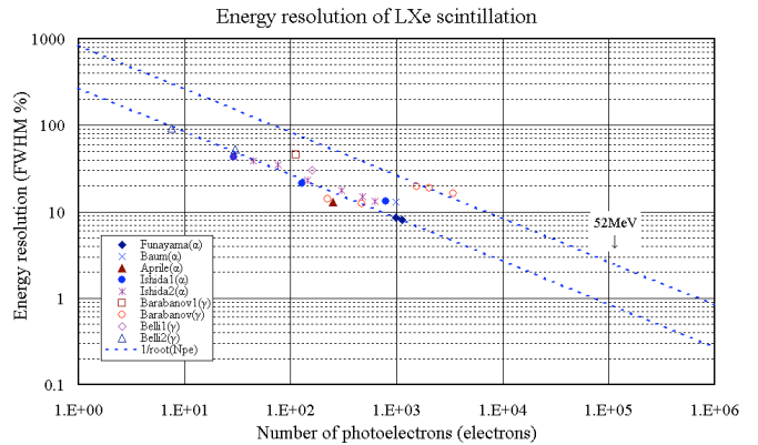
FIG. 37 Relation between energy resolutions and the estimated number of photoelectrons obtained for \alpha -particles and \gamma -rays ((Doke, 1993) and references therein.)
