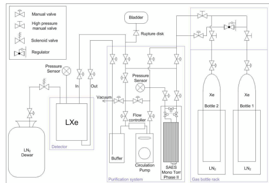
FIG. 55 The XENON10 detector purification system (Aprile, 2009).
