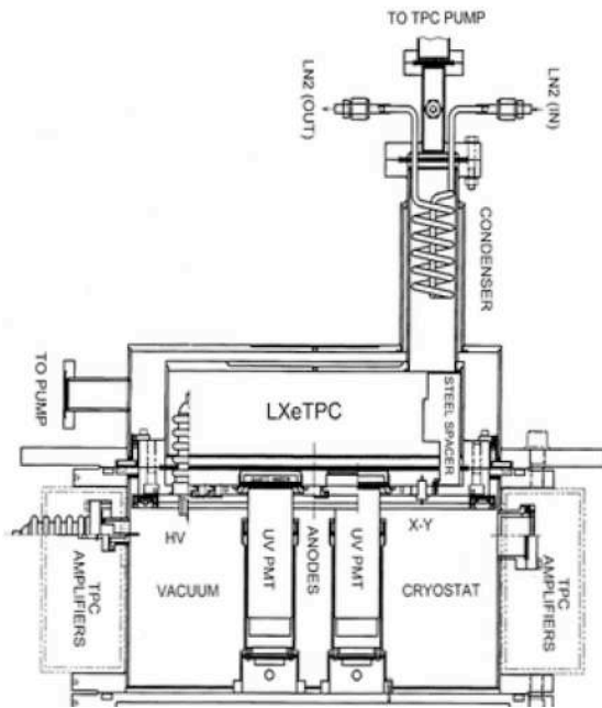
FIG. 48 Schematic of the LXeGRIT TPC (Aprile, 2003b).
