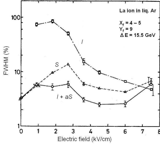
FIG. 27 Energy resolution (FWHM) of La ions in LAr as a function of the electric field, measured separately from scintillation, ionization and from their sum (Crawford, 1987).
