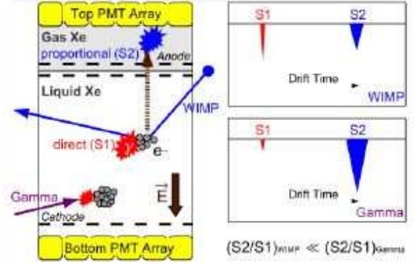
FIG. 45 Schematic of a two-phase xenon TPC.
