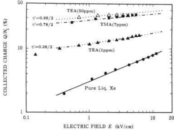
FIG. 16 Collected charge Q/N_i , where N_i is the total ionization (number of electrons) for P_\alpha \alpha -particles as a function of applied electric field. The curves represent pure liquid xenon ( \bullet ) and liquid xenon doped with TMA ( \blacksquare : 7 ppm) and TEA ( \blacktriangle : 1 ppm; \triangle : 50 ppm). The curves give the calculated results from eq. (3) in (Bakale, 1976).
