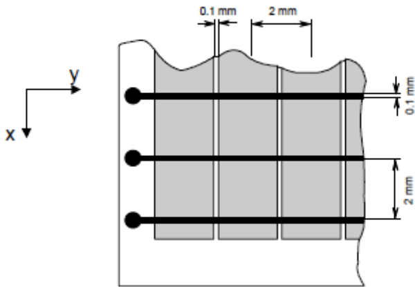
FIG. 80 The mini-strip plate of the Coimbra PET prototype (Solovov, 2002a).
