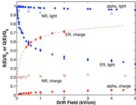
FIG. 6 Field dependence of scintillation and ionization yield in LXe for 122 keV electron recoils (ER), 56.5 keVr nuclear recoils (NR) and 5.5 MeV alphas.(Aprile, 2006).
