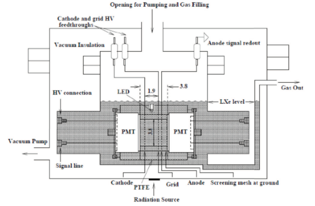
FIG. 40 Schematic of a “sum signal mode” detector (Aprile, 2007b).
