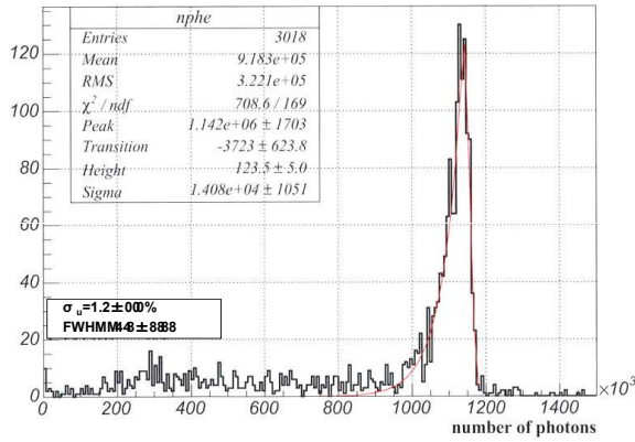
FIG. 75 Energy spectrum for 55 MeV gamma-rays measured with the large MEG prototype (Baldini, 2005a).
