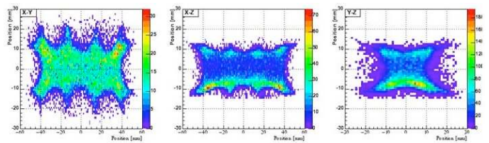
FIG. 86 Spatial distributions of 511 keV interaction points reconstructed with the Waseda prototype (Doke, 2006).
