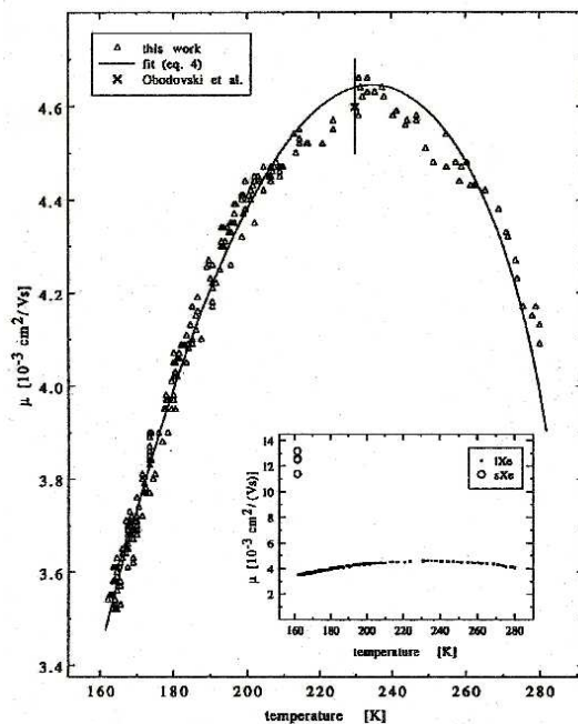
FIG. 11 Mobility of positive holes in liquid xenon as a function of temperature (Hilt, 1981).
