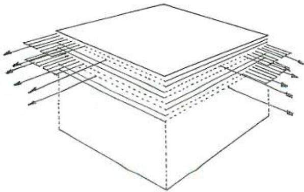
FIG. 52 Schematic of the wire electrode system for the LXe ionization calorimeter for GeV gamma rays (Doke, 1992b, 1989).
