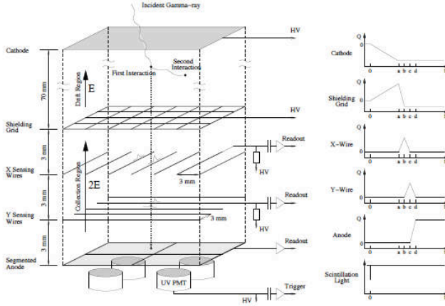
FIG. 44 Schematic of the LXeTPC electrodes structure (not to scale) with corresponding pulse shapes (Aprile, 1998).
