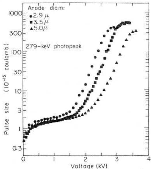
FIG. 13 Pulse height of 279 keV photopeak as a function of voltage for 2.9-, 3.5-, and 5.0- \mu\text{m} diameter anode wires (Derenzo, 1974).
