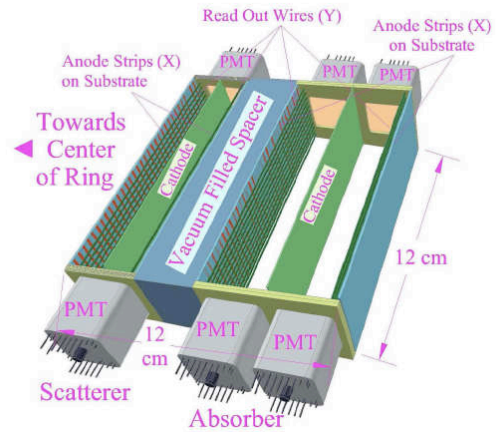
FIG. 81 Schematic of the Columbia LXe Compton PET unit cell (Giboni, 2007).
