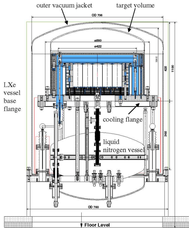
FIG. 61 Schematic of the ZEPLIN III detector (Lebedenko, 2008).
