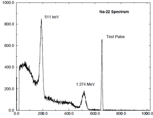
FIG. 34 The energy spectrum of Na 22 gamma-rays measured with a gridded ionization chamber (Aprile, 2001).
