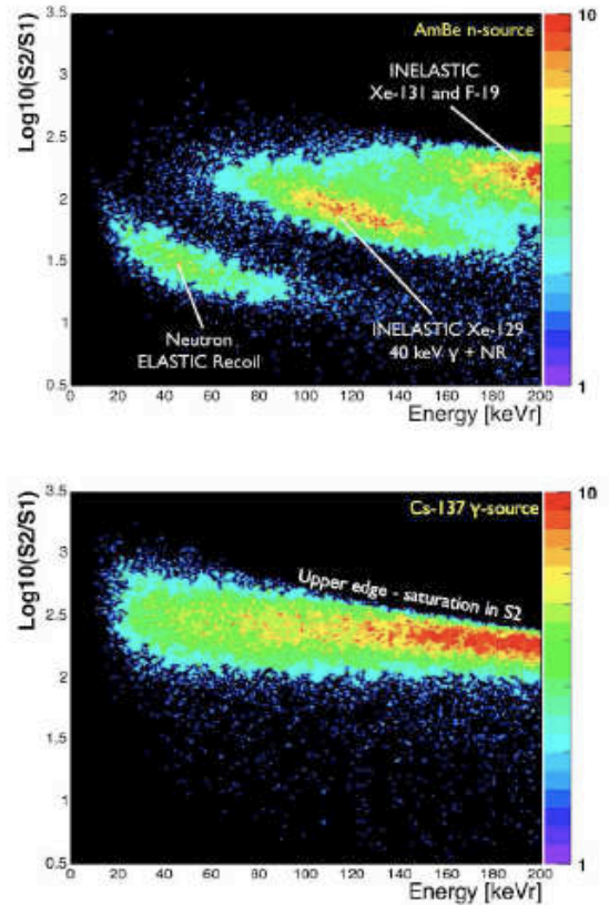
FIG. 47 A two-phase xenon detector's response to AmBe neutrons (top) and ^{137}\text{Cs} gamma rays (bottom), at 2 kV/cm drift field (Aprile, 2006).
