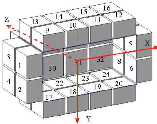
FIG. 84 Arrangement of 32 PMTs in Waseda TOF PET prototype (Nishikido, 2004).
