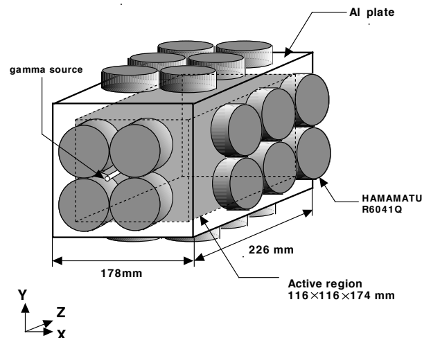
FIG. 38 Schematic of the LXe scintillation prototype with 32 2'' PMTs (Hamamatsu R6041Q) developed for the MEG experiment (Mihara, 2002).
