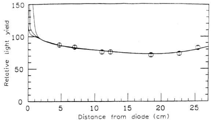
FIG. 69 Relative light yield as a function of the distance from the Si photodiode, measured with cosmic ray muons. Monte Carlo curves are shown for different light collimators (Chen, 1993).
