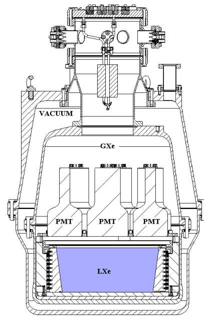
FIG. 60 Schematic of the ZEPLIN II detector (Aalder, 2007).
