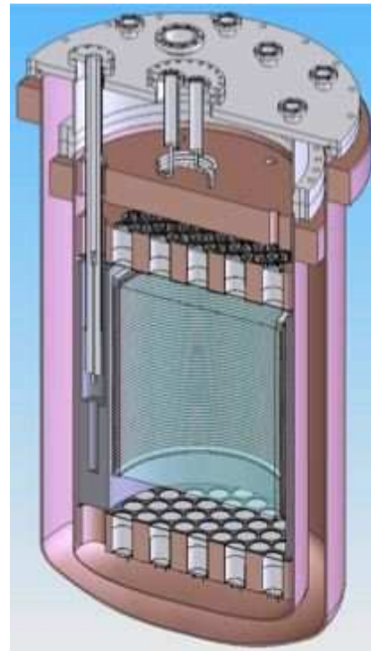
FIG. 62 Schematic of the LUX detector (Gaitskell, 2008).
