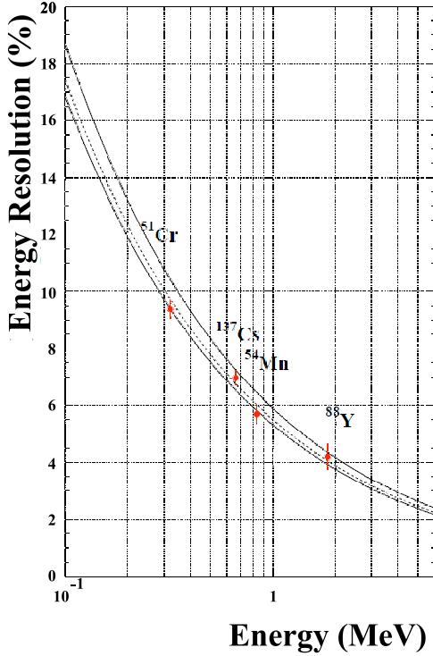
FIG. 39 Energy resolution as a function of gamma-ray energy, measured with the MEG LXe scintillation prototype. Solid curves are from Monte Carlo simulations (Mihara, 2002).
