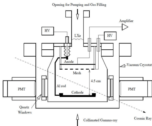
FIG. 31 Schematic of a 3.5 liter LXe gridded ionization chamber, triggered by the scintillation light (Aprile, 2001).
