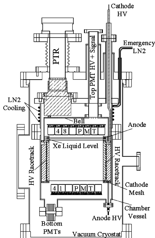
FIG. 54 Schematic of the XENON10 detector (34).
