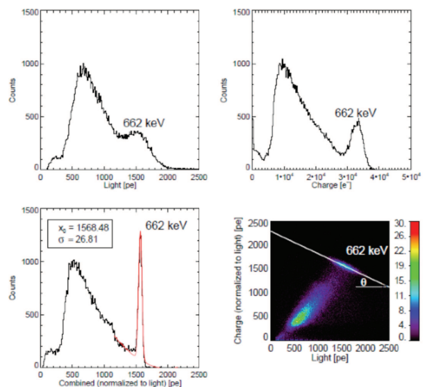
FIG. 41 Energy spectra of \text{Cs}^{137} 662 keV \gamma -rays measured with 1 kV/cm field in LXe, separately from charge and light (top panels) and from combined charge and light (lower panel, left); charge-light anti-correlation and its angle (lower panel, right) (29).
