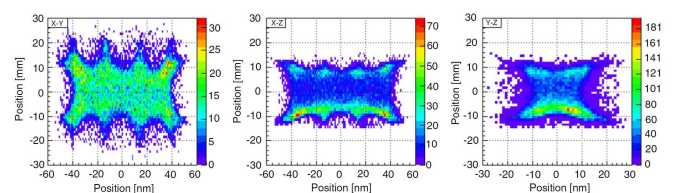
FIG. 86 Spatial distributions of 511 keV interaction points reconstructed with the Waseda prototype (113).
