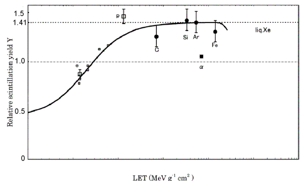
FIG. 23 LET dependence of the scintillation yield in liquid xenon for various ionizing particles (109; 237).
