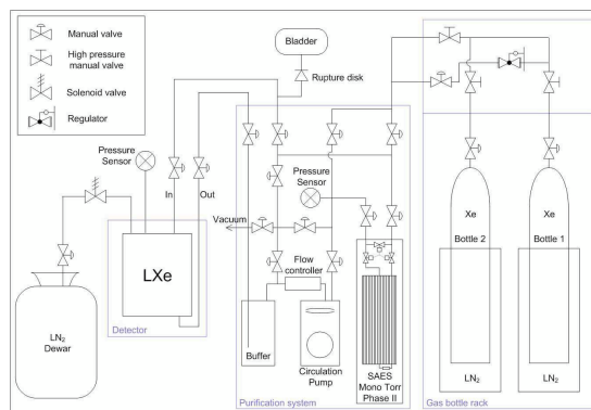
FIG. 55 The XENON10 detector purification system (34).
