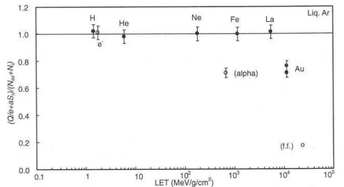
FIG. 22 LET dependence of the ratio (Q/e + aS_r)/(N_{ex} + N_i) in liquid argon. The label (f.f.) stands for fission fragments or non-relativistic particles (101; 109).
