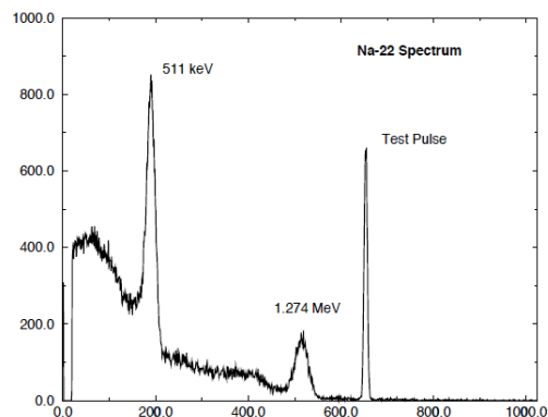
FIG. 33 The energy spectrum of \text{Na}^{22} gamma-rays measured with the gridded ionization chamber shown in Figure 30 at 4 kV/cm drift field (23). The energy resolution of the 511 keV line is about 8% (FWHM).
