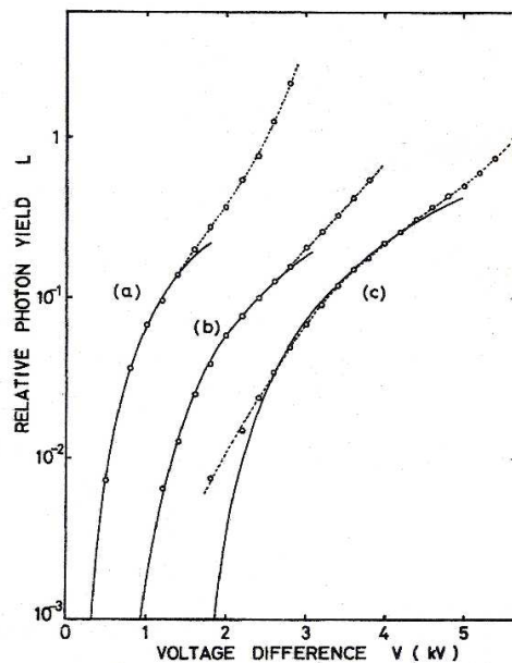
FIG. 14 Relative photon yield of proportional scintillation and charge gain as a function of applied voltage to anode wires of different diameter. Solid lines are results of the fit in (93) to the data points in the region of the ionization chamber mode: (a) for 4 \mu\text{m} diameter wire, (b) for 10 \mu\text{m} , (c) for 20 \mu\text{m} (167).
