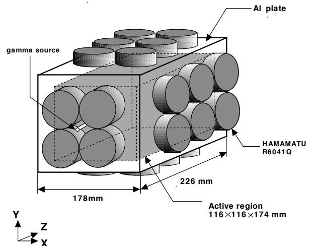
FIG. 37 Schematic of the LXe scintillation prototype with 32 2" PMTs (Hamamatsu R6041Q) developed for the MEG experiment (171).
