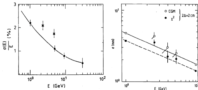
FIG. 66 (left) Energy resolution dependence on electron energy. Crosses are the experimental points and circles are points from Monte Carlo simulations. (right) Position resolution dependence on electron energy based on two different reconstruction algorithms. Full and open circles are data for two different position reconstruction algorithms, and the dashed and solid lines the corresponding predictions from simulation (50).
