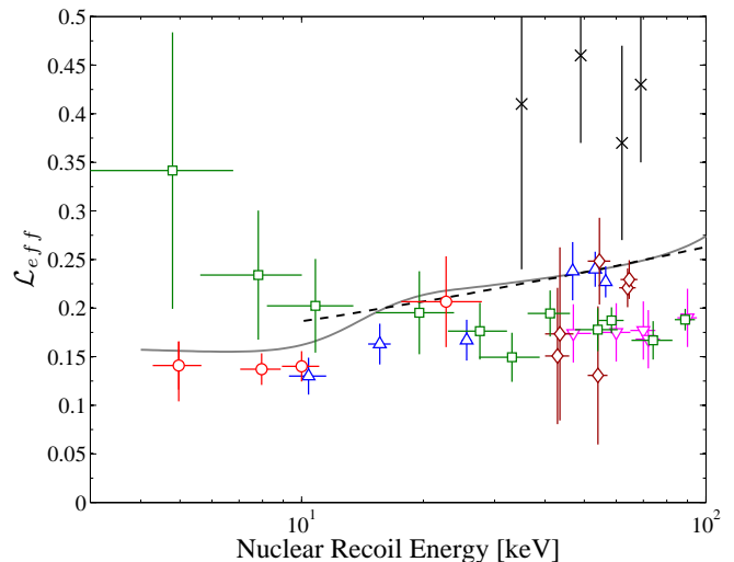
FIG. 24 Relative scintillation efficiency of nuclear recoils in LXe (32) and references therein.
