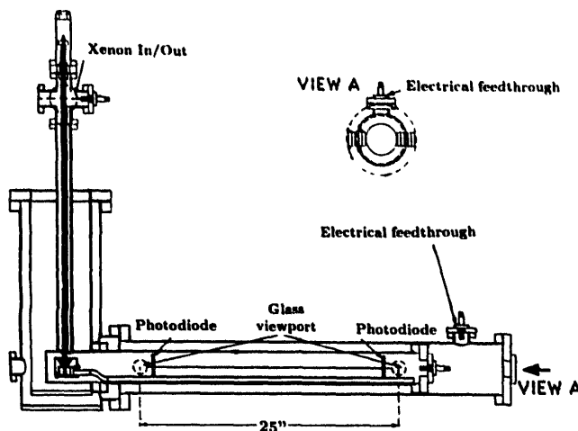
FIG. 68 Schematic of a full length liquid xenon/krypton cell for uniformity tests with mirrors and diodes (74).
