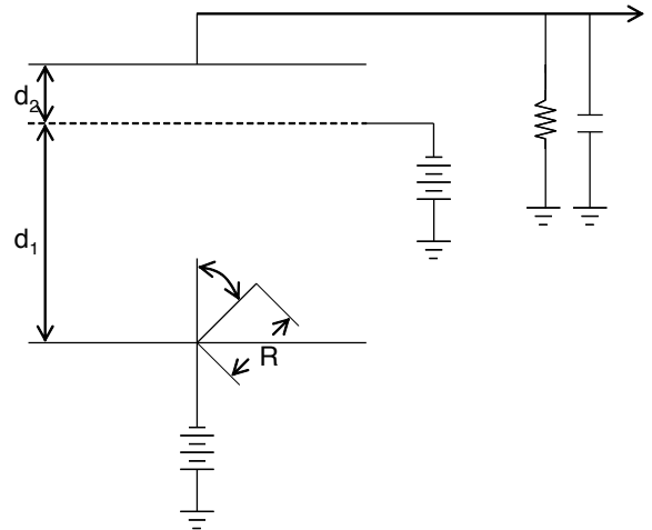
FIG. 29 Schematic drawing of a gridded ionization chamber. d_1 is the drift gap between the cathode (on the bottom) and the Frish grid, d_2 is the field region between the Frish grid and the anode (on the top).
