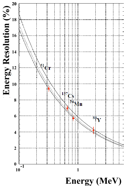
FIG. 38 Energy resolution ( 1\sigma ) as a function of gamma-ray energy, measured with the MEG LXe scintillation prototype. Solid curves are from Monte Carlo simulations (171). The data follows 1/\sqrt{N_{phe}} as expected.
