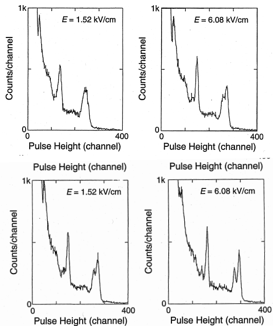
FIG. 17 Comparison between the energy spectra of ^{207}\text{Bi} internal conversion electrons and gamma-rays measured from ionization: (top) in pure liquid xenon and (bottom) in TEA-doped liquid xenon.
