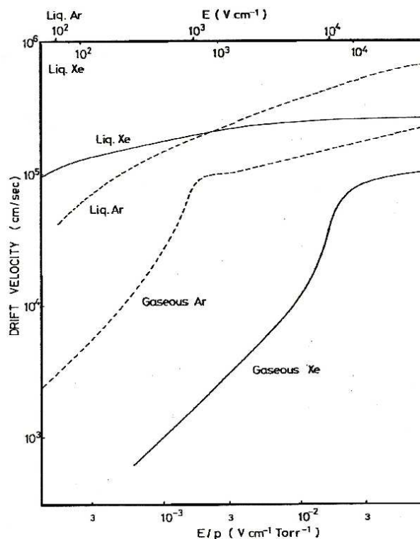
FIG. 9 Electron drift velocity in gaseous and liquid xenon and argon, as a function of reduced electric field (175; 198; 245).
