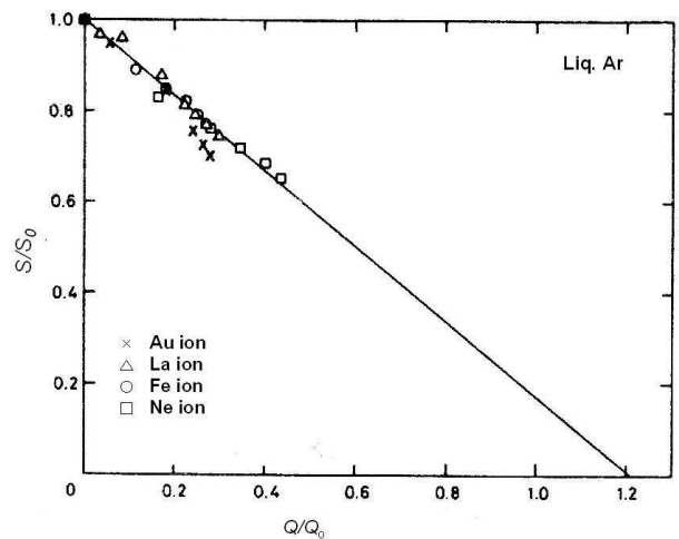
FIG. 26 Anti-correlation between scintillation intensity and collected charge in liquid argon for relativistic Ne ions( \square ), Fe ions ( \circ ), La ions ( \Delta ), and Au ions ( \times ). The solid line is the theoretically estimated relation (170).
