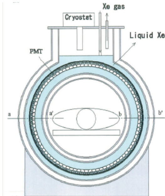
FIG. 87 Schematic of the Waseda full scale LXe TOF-PET (113).
