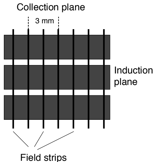
FIG. 32 An example of two-dimensional position-sensitive electrode, with orthogonal strips for collection and induction signals (72).
