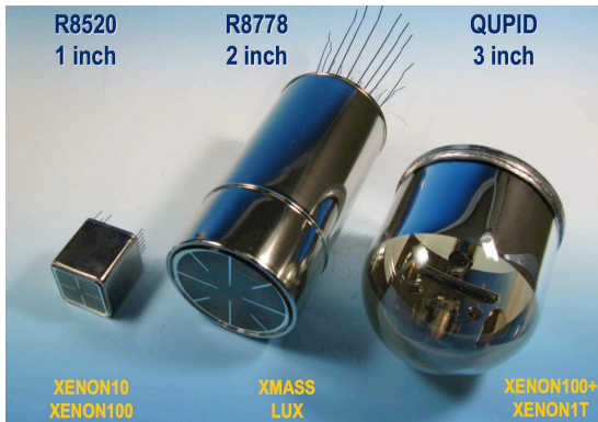
FIG. 53 A photo of the different Hamamatsu PMTs developed for the XENON and XMASS dark matter experiments.
