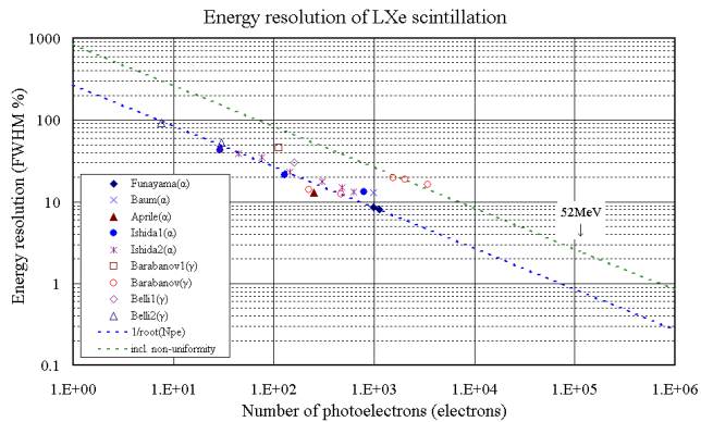
FIG. 36 Relation between energy resolutions and the estimated number of photoelectrons obtained for \alpha -particles and \gamma -rays ((107) and references therein). The lower line (blue) expresses a relation of energy resolution which is inversely proportional to the square root of the number of photoelectrons. The upper line (green) shows a worse energy resolution expected from the non-uniformity of light collection.
