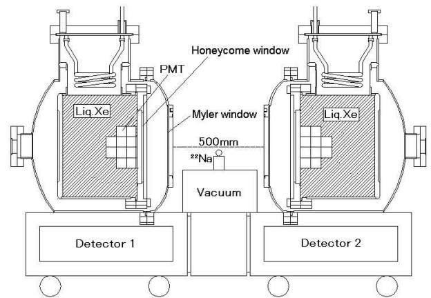
FIG. 85 Schematic of the Waseda TOF PET prototype (189).
