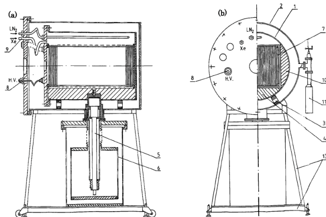
FIG. 65 (a) and (b), Schematic of the Russian LXe ionization calorimeter: inner (1) and outer (2) cylindrical vessel, (3) multi-plate supports, (4) and (10) aluminum segments, (5) copper bar, (6) cryostat with \text{LN}_2 , (7) electrode system, (8) HV connector, (9) Xe gas supply tube, (11) zeolite trap (50).
