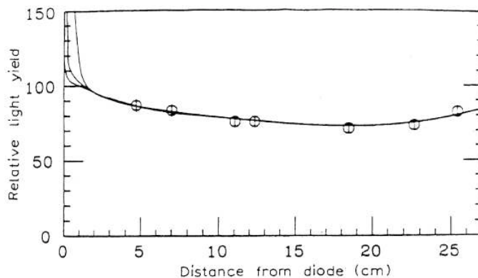
FIG. 69 Relative light yield as a function of the distance from the Si photodiode, measured with cosmic ray muons. Monte Carlo curves are shown for different light collimators (74).
