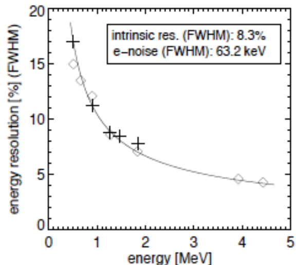
FIG. 50 The energy resolution of LXeGRIT as a function of energy, as measured during two different balloon flights (crosses and diamonds).
