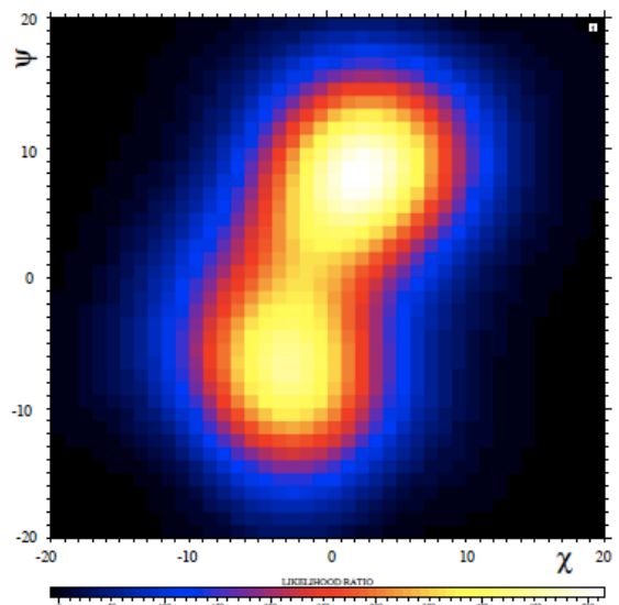
FIG. 51 LXeGRIT image (reconstructed angles in degrees) of two calibration sources, ^{60}\text{Co} and ^{22}\text{Na} , using a maximum likelihood imaging technique. Reprinted with permission from (30).
