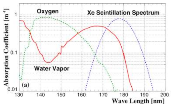
FIG. 25 Absorption coefficient for VUV photons in 1 ppm water vapor and oxygen and superimposed Xe emission spectrum (197).
